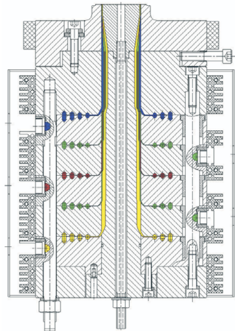
Modular lab die for film development
